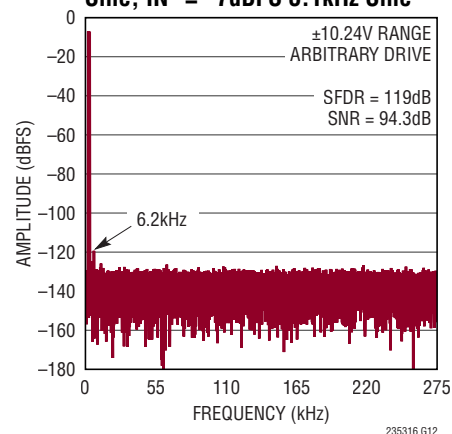
32k Point Arbitrary Two-Tone FFT f_{SAMPL} = 550\text{ksps} , IN^+ = -7\text{dBFS } 2\text{kHz} Sine, IN^- = -7\text{dBFS } 3.1\text{kHz} Sine
